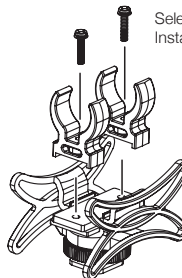
Mounting Base
